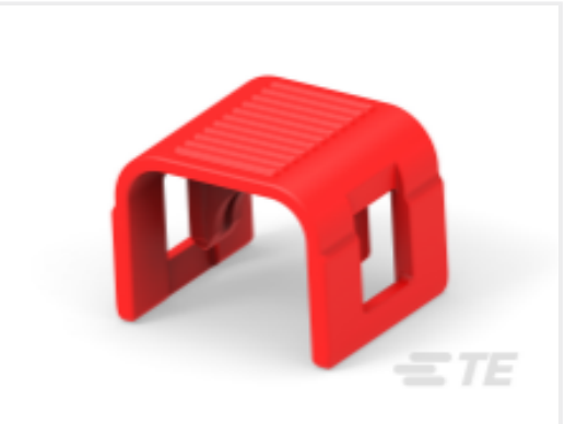
TE 产品编号1438888-1 LOCK, JACK, 1 POSITION, 180 DEGREE, FAKR
