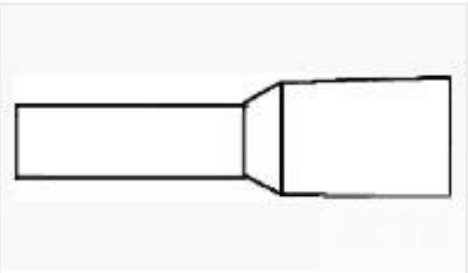
TE 产品编号1-966067-6 FER,WIRE,PL SLV,2.50/14,L8,BLUE,LP
