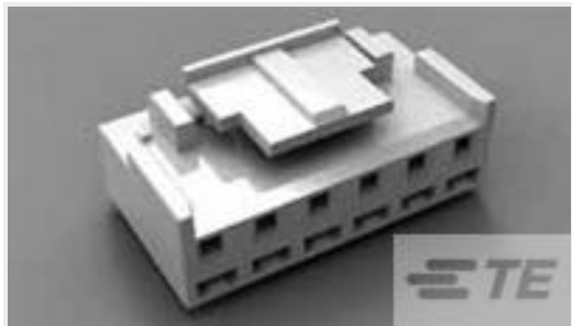
TE 产品编号4-1123722-5 3.96 EP PLUG HSG 5P(RED)
