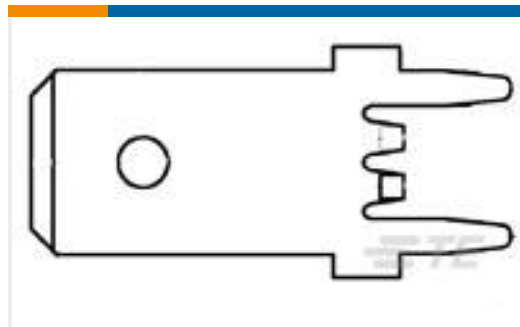
TE 产品编号1217169-1 250 FASTON,PCB TAB,TCBR
