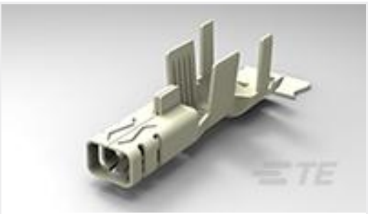
TE 产品编号1971781-2 PTL RECEPTACLE CONTACT, 14 AWG
