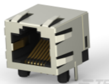
TE 产品编号1775134-4 MOD JACK, RJ45, SINGLE, 50u" Au"
