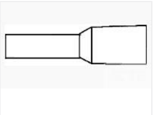
TE 产品编号1-966067-2 FER,WIRE,PL SLV,1.50/16,L8,BLACK,LP
