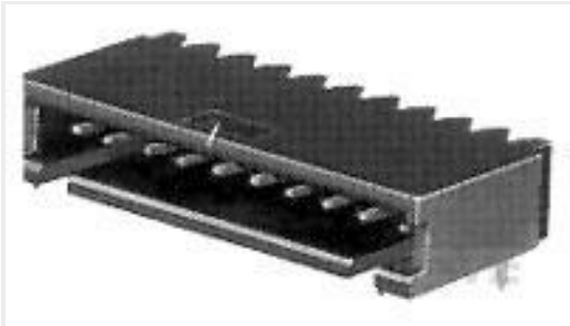
TE 产品编号5-102203-3 06 MODII HDR SRRA SHRD LF
