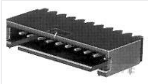
TE 产品编号5-102523-1 04 MODII HDR SRRA SHRD .100CL
