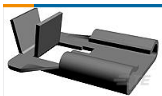
TE 产品编号63508-1 250 FASTON FLAG REC 18-14 AWG BR
