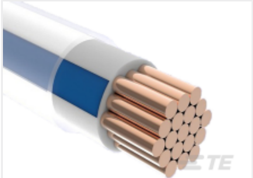
TE 产品编号0297023001 ACW0219-0.50-1(NS)
