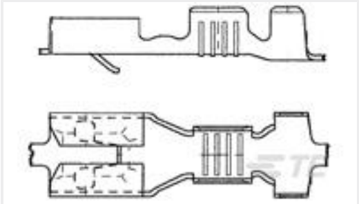
TE 产品编号282180-1 FF 187 REC 0.5-1.5MM2 TPBR
