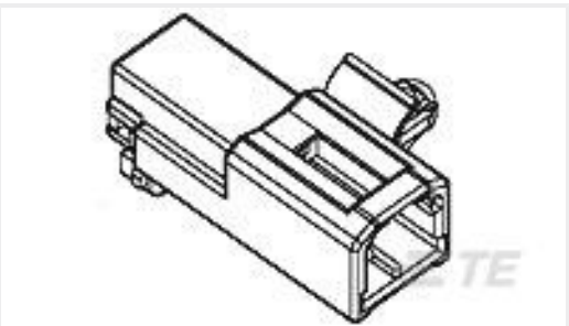
TE 产品编号85284-1 070 MLC 2P CAP HSG(CLIP TYPE)
