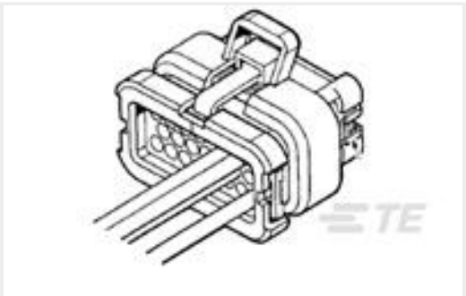
TE 产品编号776273-1 14POS,AMPSEAL,SOC HSG ASSY,SLD, COD 1
