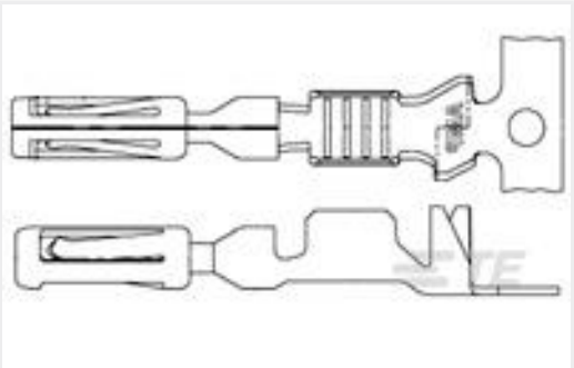
TE 产品编号770520-1 AMPSEAL,TERMINAL,TIN PLATE,16-20AWG WIRE
