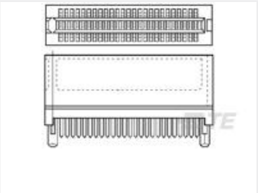
TE 产品编号5650719-2 STANDARD EDGE .050 SERIES 25 DUAL ASSY
