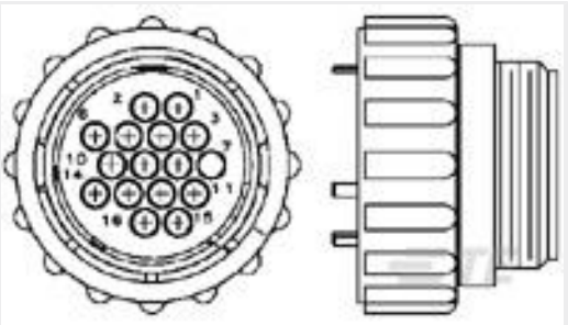
TE 产品编号206037-3 CPC PLUG ASSEMBLY SZ 17-16
