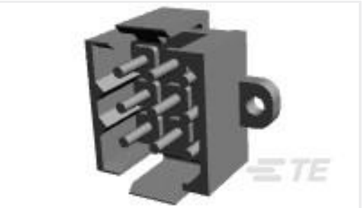
TE 产品编号207441-7 METRIMATE PIN HEADER ASSY,9P
