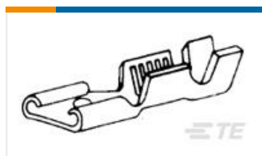
TE 产品编号60384-1 .250 FAST REC IS 1000 BR
