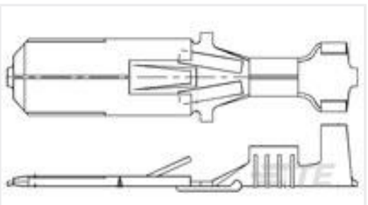
TE 产品编号170151-2 FF 250 TAB 18-14AWG PTBR
