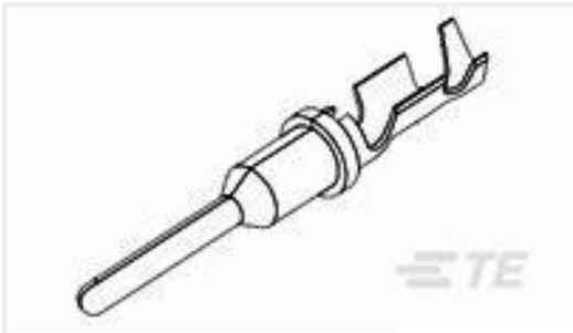
TE 产品编号638078-1 PIN, SF, SIZE 16, 14-18 AWG, AU/SN
