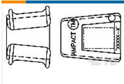
TE 产品编号602007 AMPACT Tap 336.4-336.4
