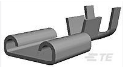
TE 产品编号170179-2 205 FASTON,REC.,18-14 AWG,TPBR
