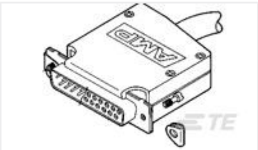
TE 产品编号5206478-5 CLAMSHELL SIZE 5 W/RETAINER
