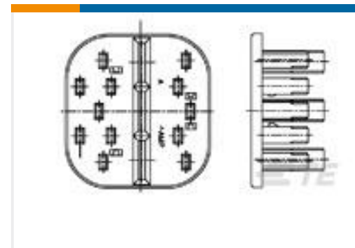
TE 产品编号85223-1 E-J MK-II(+) 15P PLUG DBL
