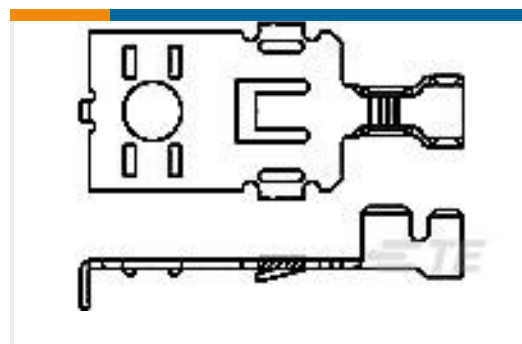
TE 产品编号63496-1 POWER RING TERMINAL TAB 16-10 AWG BR
