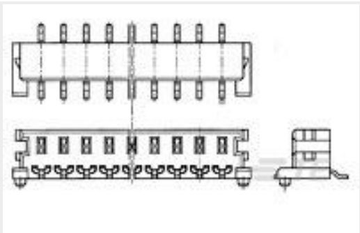
TE 产品编号7-917570-2 1.5 B-T-W HDR ASSY 12P W/O BOS
