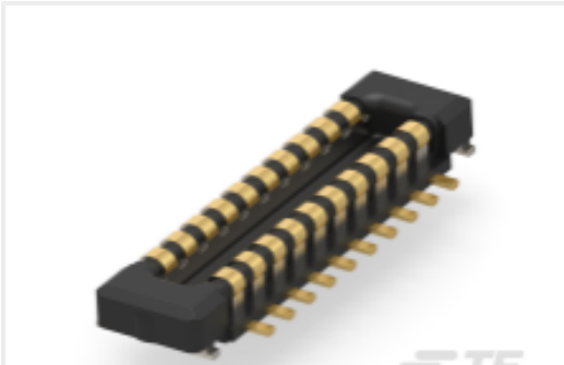
TE 产品编号2-2363962-0 0.4mm BTB CONN H0.8 PLUG ASSEMBLY, 20P
