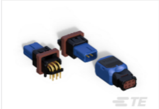
TE 产品编号YD369-B99-AP400000 369 9 WAY PANEL MNT REC, 90 PCB GOLD,PIN
