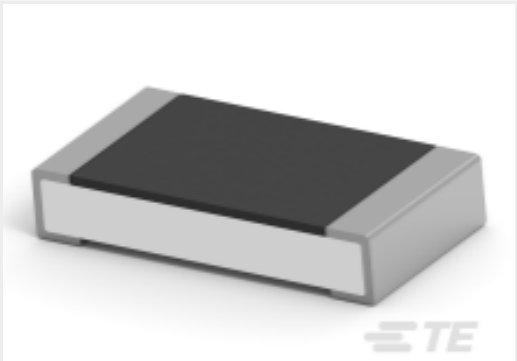
TE 产品编号5-2176390-3 RQ 1206 4K02 0.1% 10PPM 5K RL
