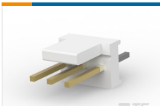
TE 产品编号640454-3 PCB Header: Polyester, Vertical, 2.54 mm
