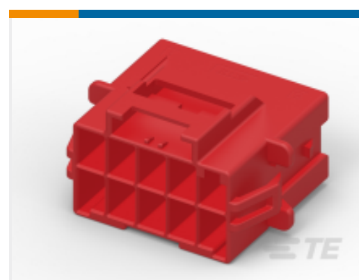
TE 产品编号 6-1971775-5 PTL 2X5 CAP PANEL MT HIGH TEMP KEY B RED
