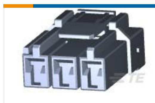
TE 产品编号1747995-1 GHC EYELET 6.2 3POS PLUG HOUSING NATURAL
