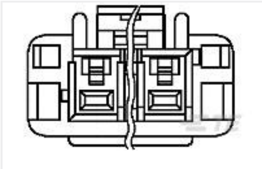
TE 产品编号1-1376388-2 5MM POWER KEY 2P PLUG HSG RED
