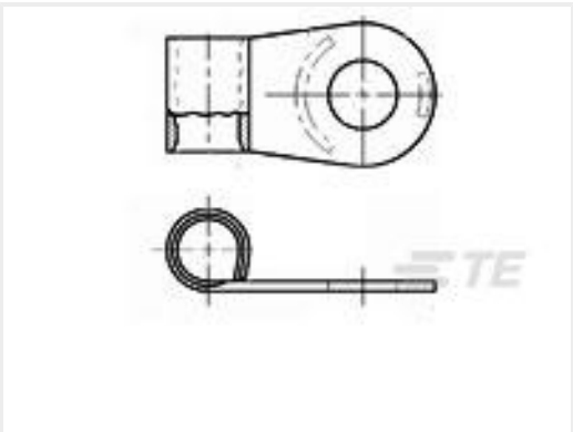
TE 产品编号321060 TERMINAL,SOLIS FLAG R 4 5/16
