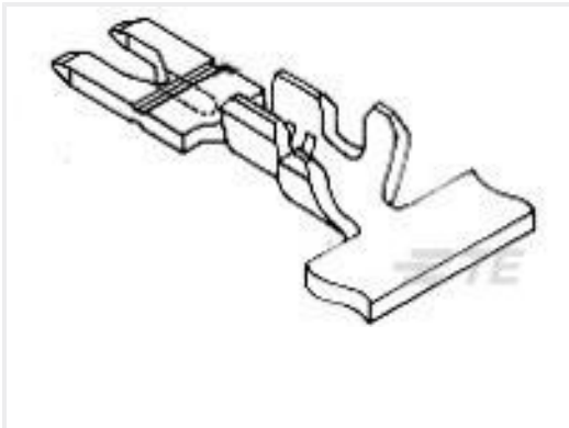
TE 产品编号63397-1 MAG-MATE POKE-IN TAB 0198 TPBR
