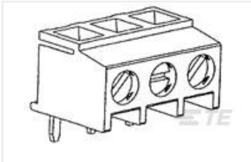
TE 产品编号284093-6 TERMI-BLOK PCB MOUNT 90, 5,0MM
