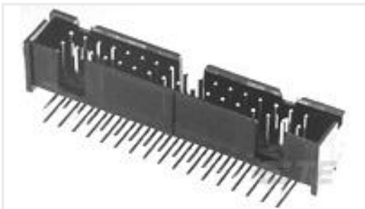
TE 产品编号5103311-3 A/L LOW PRO HDR 16P RA BLACK
