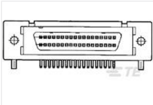
TE 产品编号2-5174225-5 AMPLIMITE 050-2B HOR 68P M2.5
