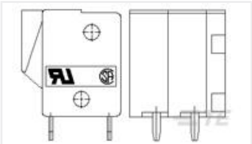
TE 产品编号1776259-2 2P Spring TB, 180deg, VT,5mm, Green
