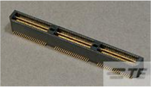
TE 产品编号 4-1658014-3 MSB0.80PL8ASY120FL,GP,10,-TR
