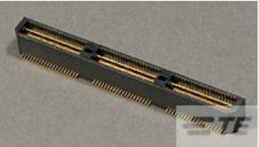
TE 产品编号 6-1658045-3 MSB0.80PL8ASY120FL,GP,F,-TR
