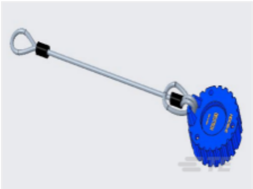
TE 产品编号HDC16-6-LA DUST CAP, 6P, REC, GRY, LANYARD, HD10
