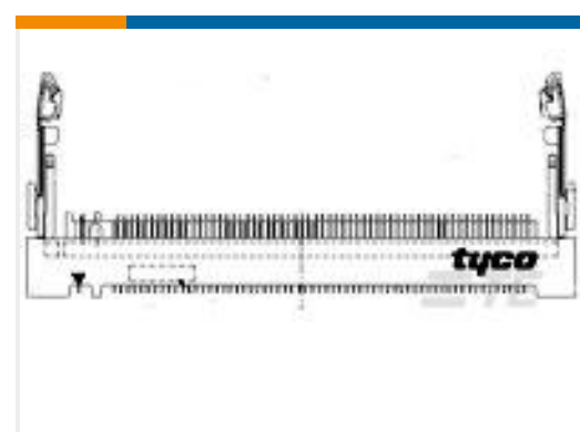
TE 产品编号440360-2 .8MM FAX MODEM SOCKET 124P, 7.95H
