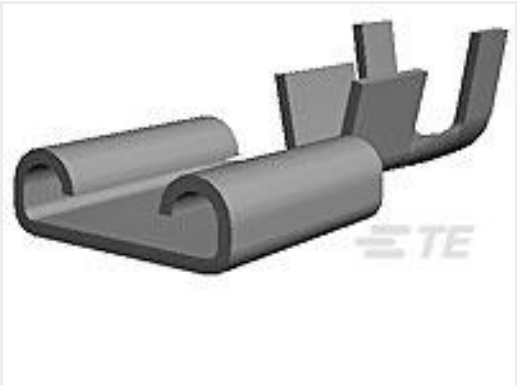
TE 产品编号140760-2 250 FASTON, REC., 22-18 AWG, TPPB
