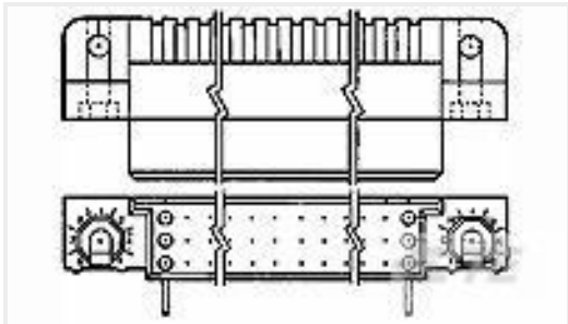
TE 产品编号5533268-3 ASSY,RECPT,R.ANGLE,HDI,LEAD-FR
