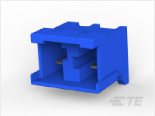
TE 产品编号1-1747052-3 GIC7.92 2POS_HEADER ASS'Y BLUE KEYING B
