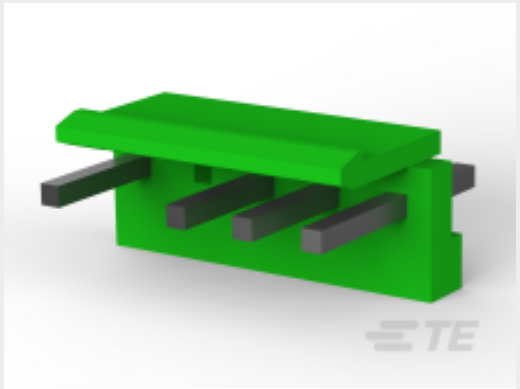
TE 产品编号 6-1717011-4 EP CONN.HDR ASSY 4/5POS-W/O NO.2
