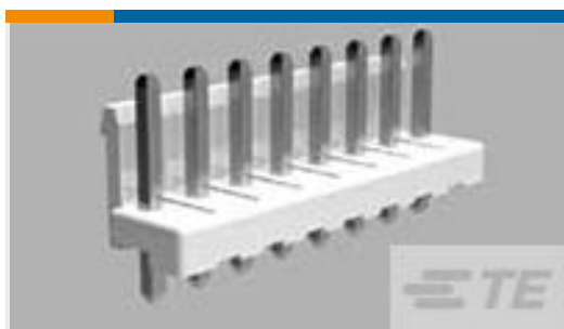
TE 产品编号4-1123723-3 3.96 EP HDR ASSY 3P(RED)
