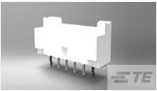
TE 产品编号2132415-4 EP2.5 Shrouded HDR ASSY 4P VERT w /o boss
