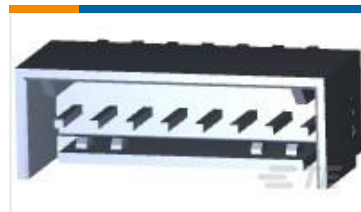
TE 产品编号2-644861-8 08P MTA100 SHRD HDR,W/O PEG SN
