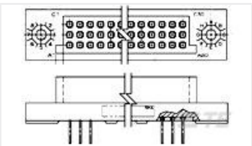
TE 产品编号446853-1 3 ROW BOX REC 90P 100CL SEALED
