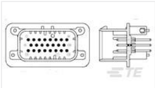
TE 产品编号776230-2 35POS,PIN DIA 1.3,HDR ASSY, 180DEG,COD 2
