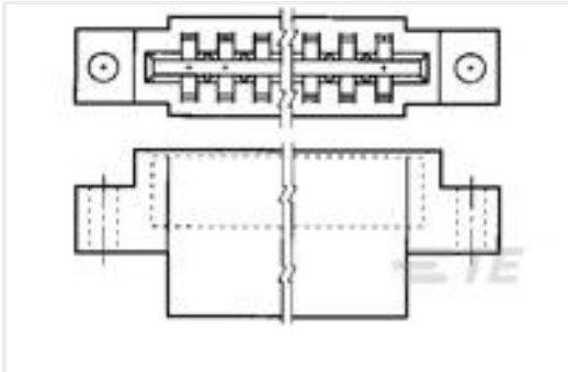
TE 产品编号2-583859-3 HOUSING
