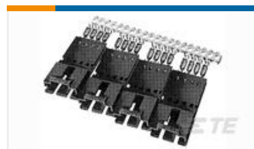
TE 产品编号 5-103945-6 3X7 MTE SHRD PIN SR LATCH .100
