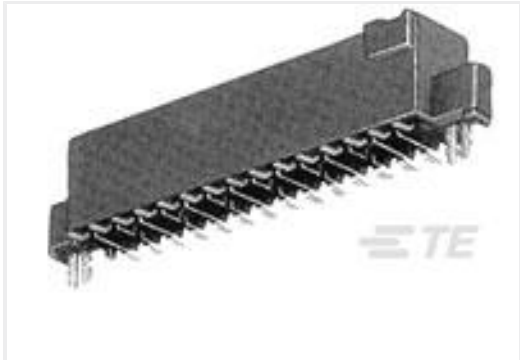
TE 产品编号5-104652-4 40 50/50 GRID DRST SFMNT RCPT
